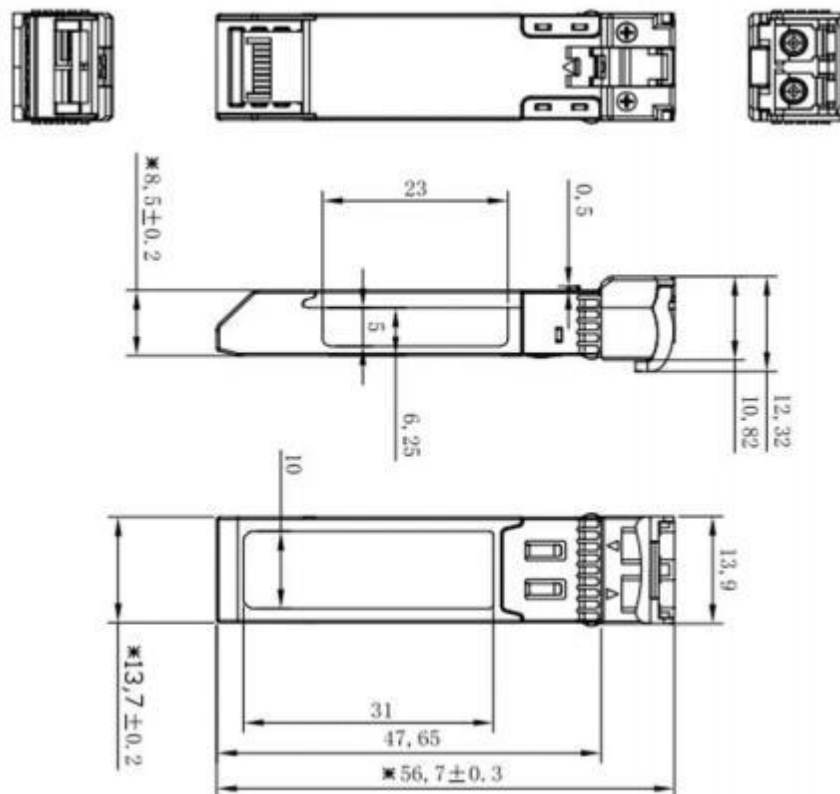
SFPwiremechanicaldrawing (Unit:mm)
